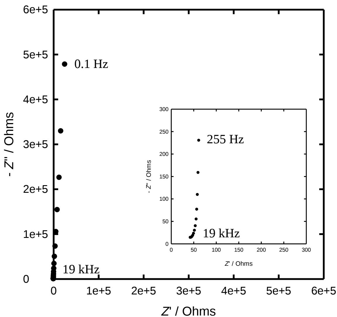
Fig. S1 Nyquist plot for the H 1 mesoporous platinum film electrodeposited onto a Pt disc electrode (deposition charge = 6.27 mC, 500 \mu m in diameter) in 1 M H 2 SO 4 at –0.25 V vs. SMSE. Inset: zoom at high frequencies.
