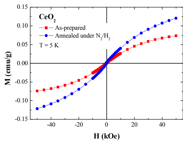
Magnetization curves recorded at 5 K of CeO 2 as-prepared and annealed under N 2 /H 2 .
