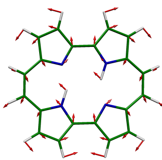
1 BU, 237 \text{cm}^{-1}
