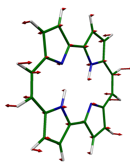
6 BG, 493 \text{cm}^{-1}
