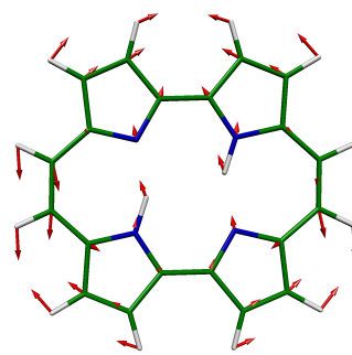
5 BU, 626 \text{cm}^{-1}
