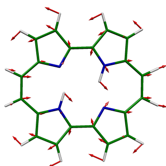
4 BU, 472 \text{cm}^{-1}
