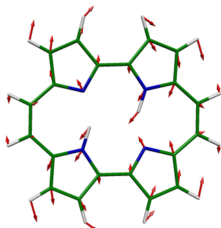
2 BU, 323 \text{cm}^{-1}
