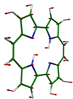
11 BG, 775 \text{cm}^{-1}
