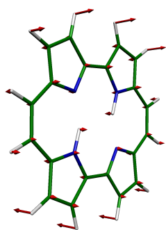
12 BG, 789 \text{cm}^{-1}
