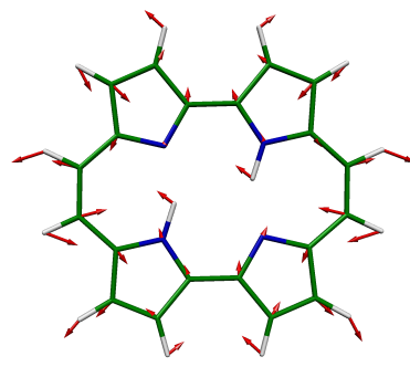
7 BU, 836 \text{cm}^{-1}
