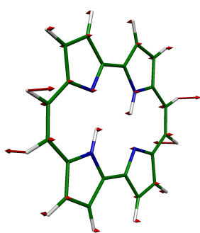
17 BG, 958 \text{cm}^{-1}
