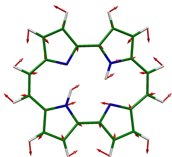
11 BU, 1028 \text{cm}^{-1}
