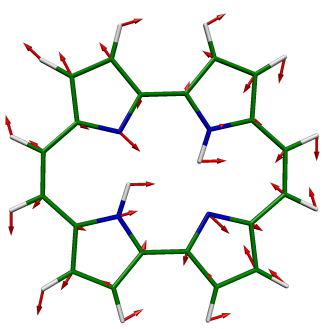
10 BU, 965 \text{cm}^{-1}
