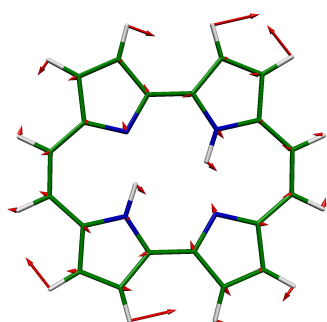
12 BU, 1075 \text{cm}^{-1}
