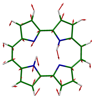
9 BU, 947 \text{cm}^{-1}
