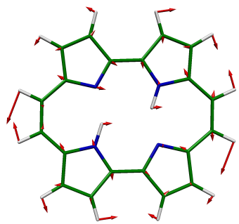
16 BU, 1227 \text{cm}^{-1}
