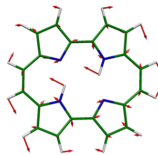
17 BU, 1270 \text{cm}^{-1}
