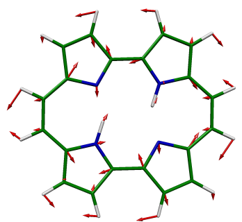
18 BU, 1285 \text{cm}^{-1}
