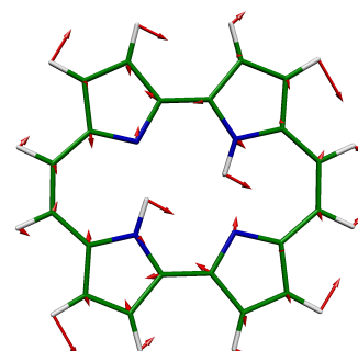
14 BU, 1122 \text{cm}^{-1}
