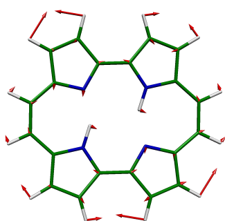
13 BU, 1087 \text{cm}^{-1}
