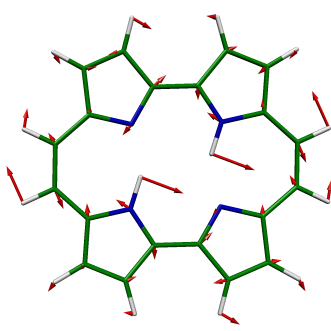
26 BU, 1531 \text{cm}^{-1}
