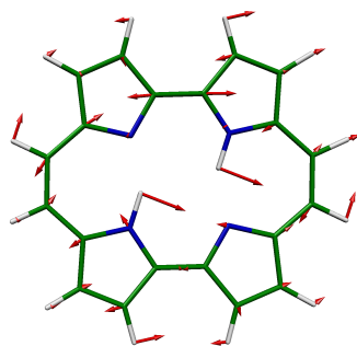
28 BU, 1617 \text{cm}^{-1}
