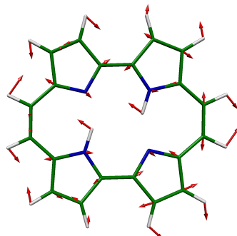
27 BU, 1571 \text{cm}^{-1}
