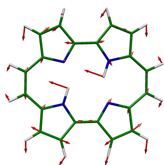
25 BU, 1516 \text{cm}^{-1}
