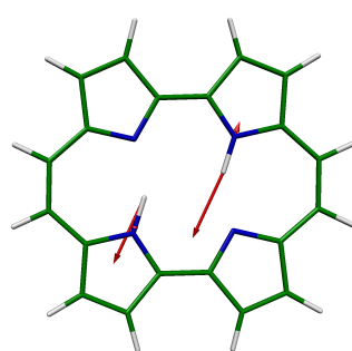
30 BU, 2895 \text{cm}^{-1}
