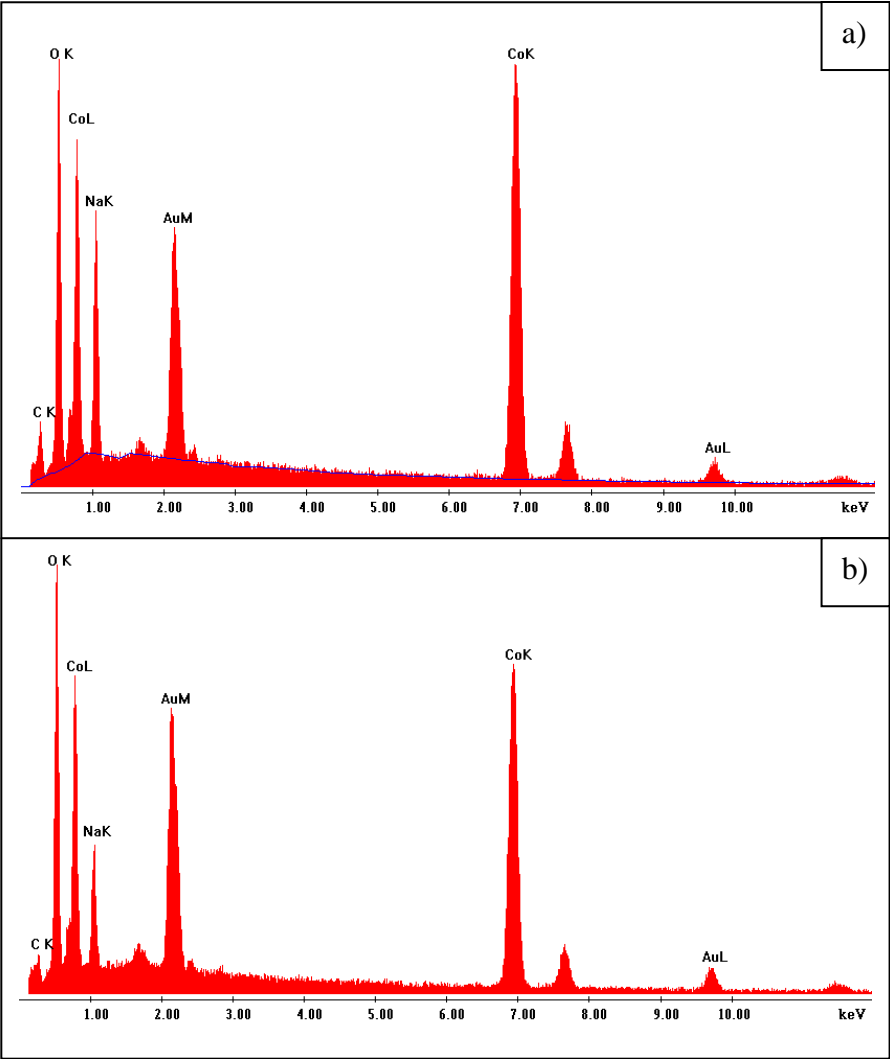
Fig. S1: EDX spectra of a) Na 0.71 CoO 2 (I) and Na 0.71 CoO 2 (II)
