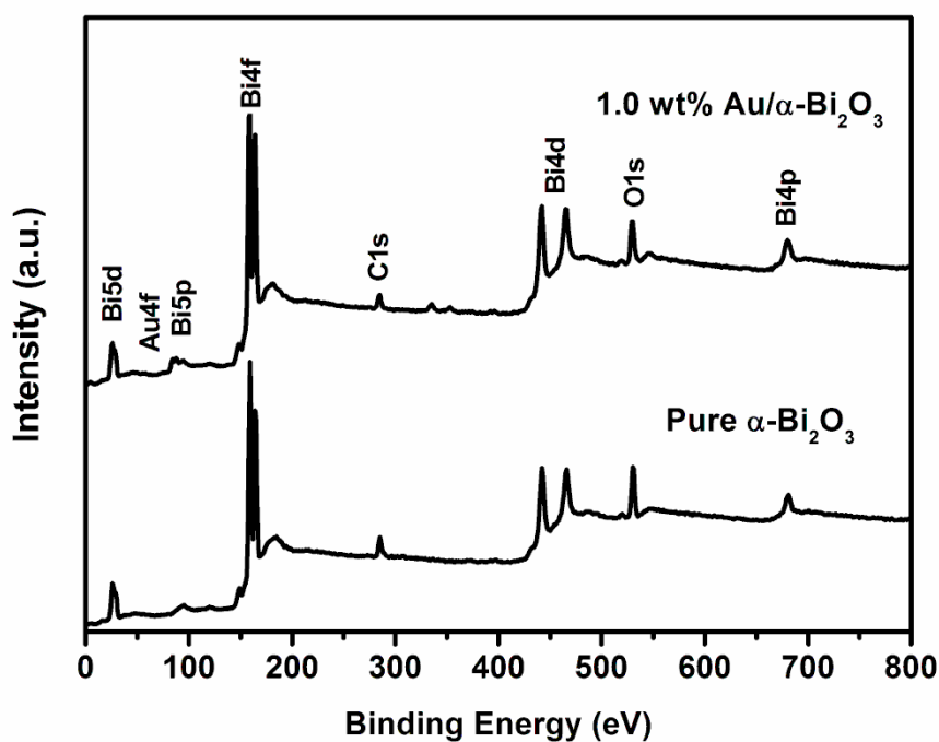
Fig. 1S XPS survey spectra for the surface of pure \alpha - \text{Bi}_2\text{O}_3 and 1.0 wt% Au/ \alpha - \text{Bi}_2\text{O}_3 .
