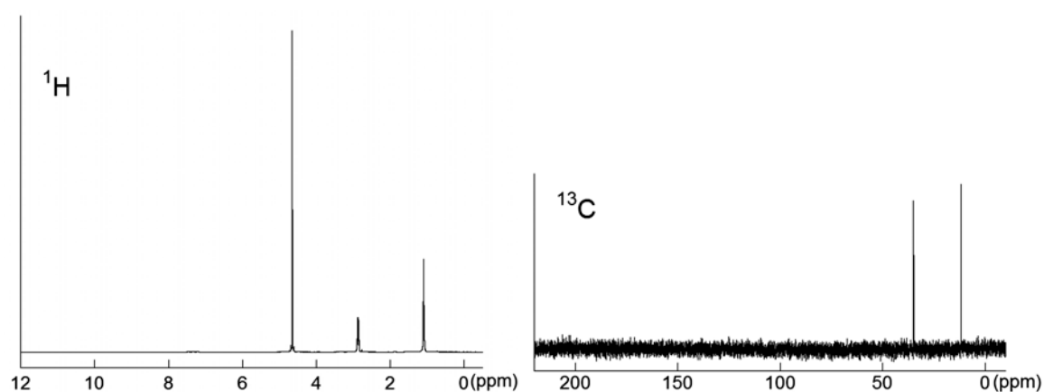
Figure S1. 1 H and 13 C NMR data for EtNH 3 NO 3 in CD 3 CN.
