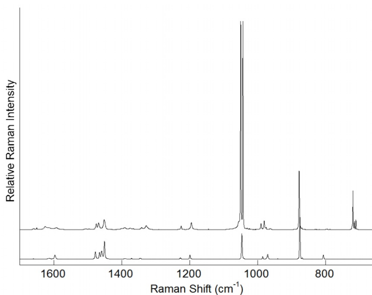
Figure S2. Raman spectra of (top) EtNH 3 NO 3 and (bottom) EtNH 3 Cl.
