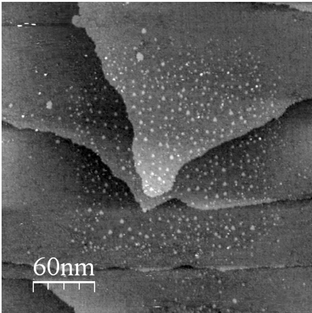
300 nm x 300 nm STM image of the network sample on Au-surface imaged after continuous high voltage (-1V) scanning was performed on 200 nm x 200 nm area. The inner area contains particles and disrupted material caused by high voltage imaging.
