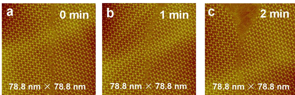
Figure S1. Sequential STM images of a 78.8 nm × 78.8 nm region illustrating the change process of the structure of phase (I) with time ( V = -531.4 mV, I = 518.8 pA ). The time of the first image is arbitrarily set to zero.
