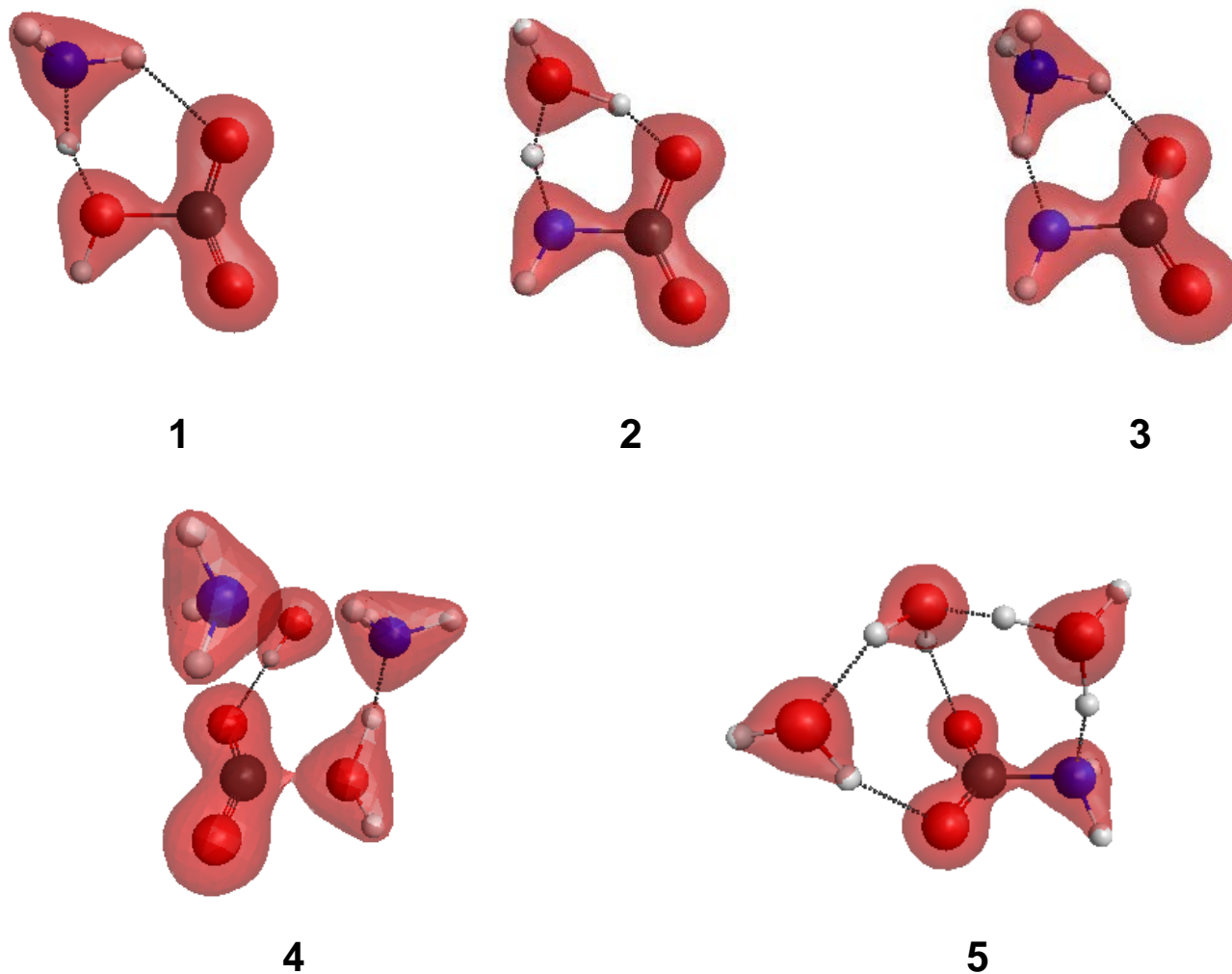
Figure S1. Electron pair density plots for selected TS's from LMO calculations. In some cases, the plots indicate N-CO 2 or O-CO 2 bond formation slightly precedes transfer of the proton to the acceptor e.g. 2,4,5 ; in other cases (1 and 3), it is almost simultaneous. In any case, the entire process is completed within one vibration.
