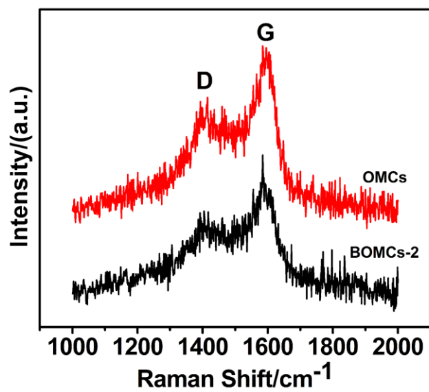
Fig. S2 Raman spectra of OMCs (red line) and BOMCs-2 (black line).
