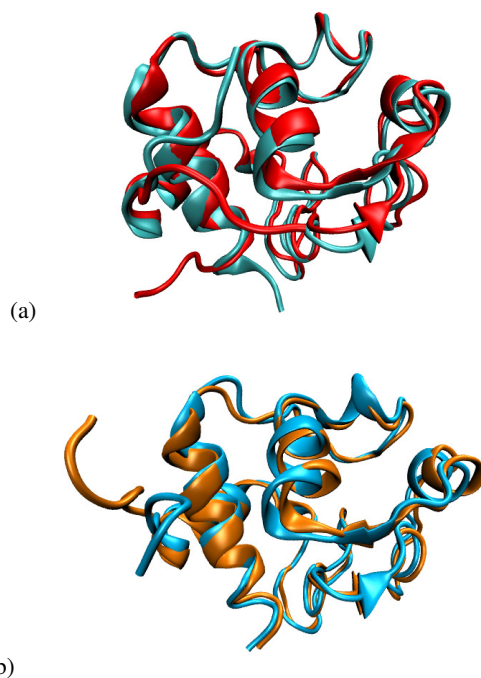
Figure S1. Comparison between the protein structures in the final snapshots of the simulations. Panel (a) native YCC in water (cyan) and on gold (red). Panel (b) N67C mutant in water (light-cyan) and on gold (orange).
