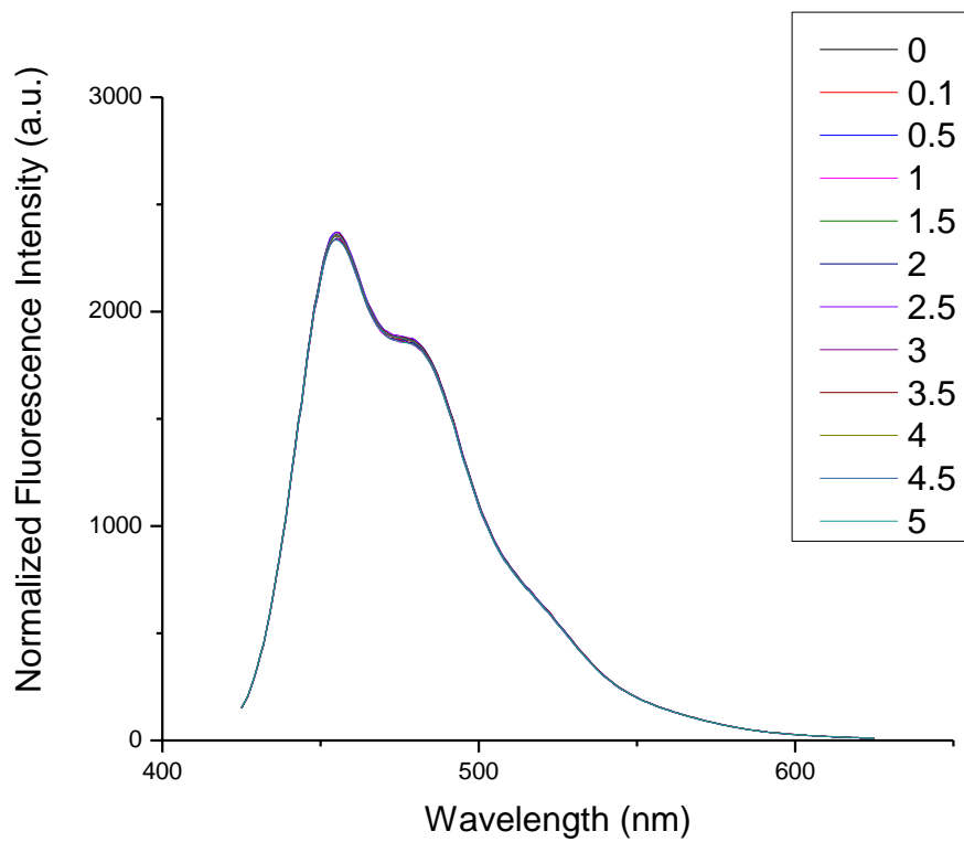
Figure 3. Normalized fluorescence intensity for toluene experiments.
