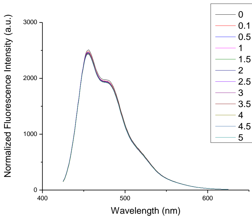
Figure 2. Sample fluorescence spectra for nitrobenzene experiment. The fluorescence intensity is normalized with the absorbance data.
