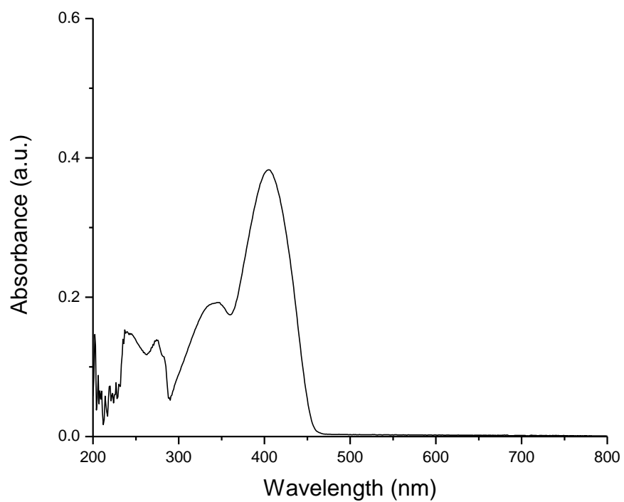
Figure 1. UV/VIS spectrum of OPV
