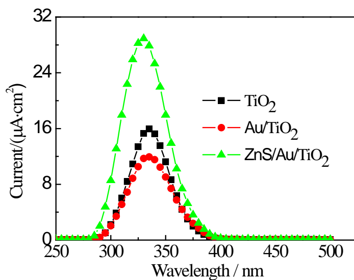
Fig.S1 Photocurrent spectra of photoanodes with different nanotube films
