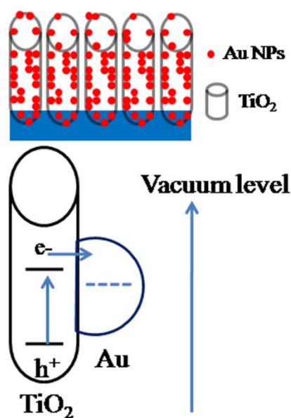
Fig. S3 Schematic diagrams of charge transfer mechanism in the Au/ \text{TiO}_2 nanotube array film.
