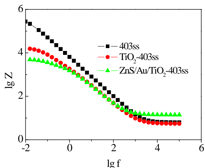
Fig. S2 The EIS results Bode- |Z| versus frequency.
