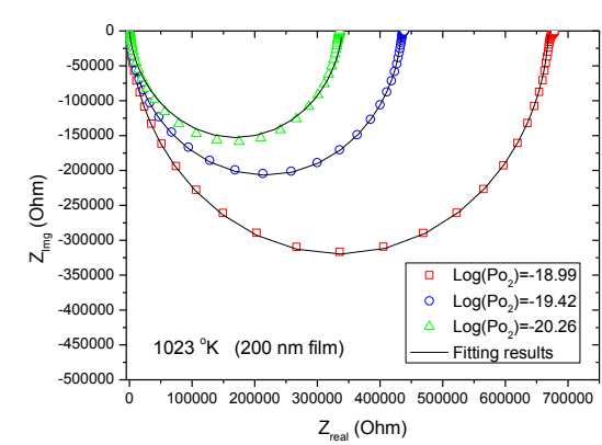
Figure S1. Typical impedance spectra of ceria film and their fitting results using single R-C (resistance-capacitance) parallel equivalent circuit.
