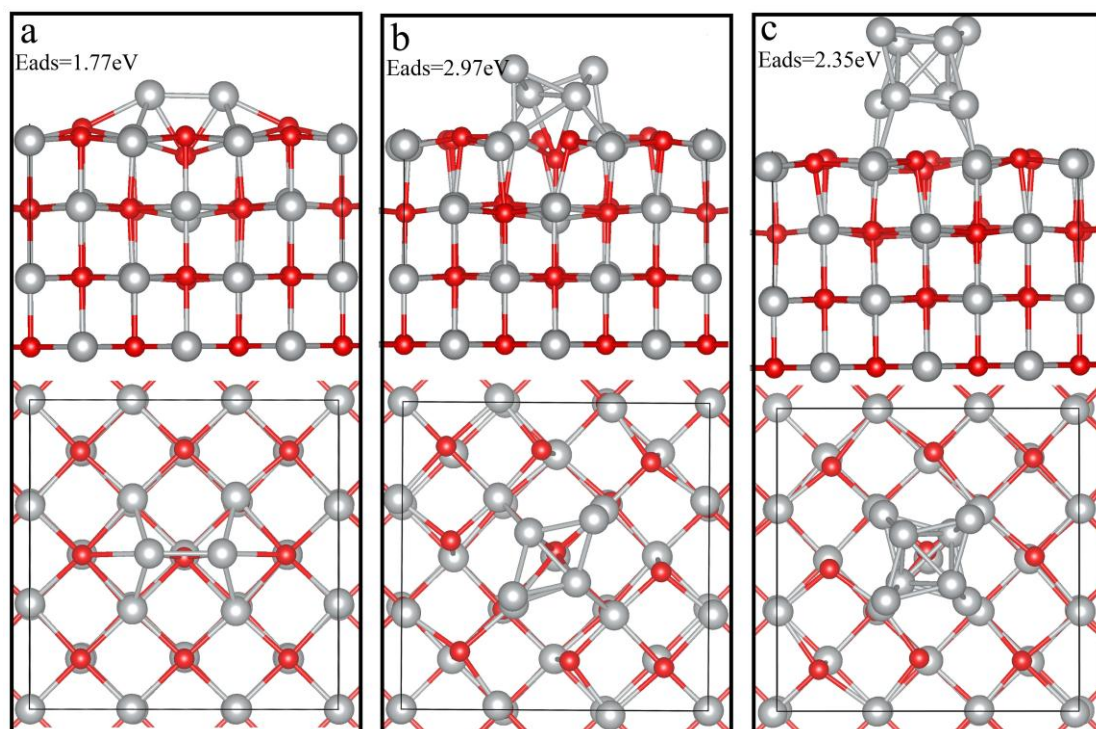
Figure S1. The second most stable adsorption configurations of (a) Ag 2 , (b) Ag 4 and (c) Ag 8 clusters on the AgCl (100) surface along with the respective adsorption energy (Eads).
