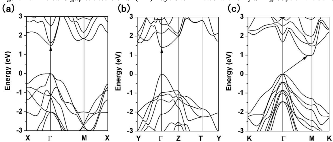
Fig.2s Band gap structure of (a) (100) monolayer, (b) (110) monolayer, (c) (111) monolayer without structural optimization
