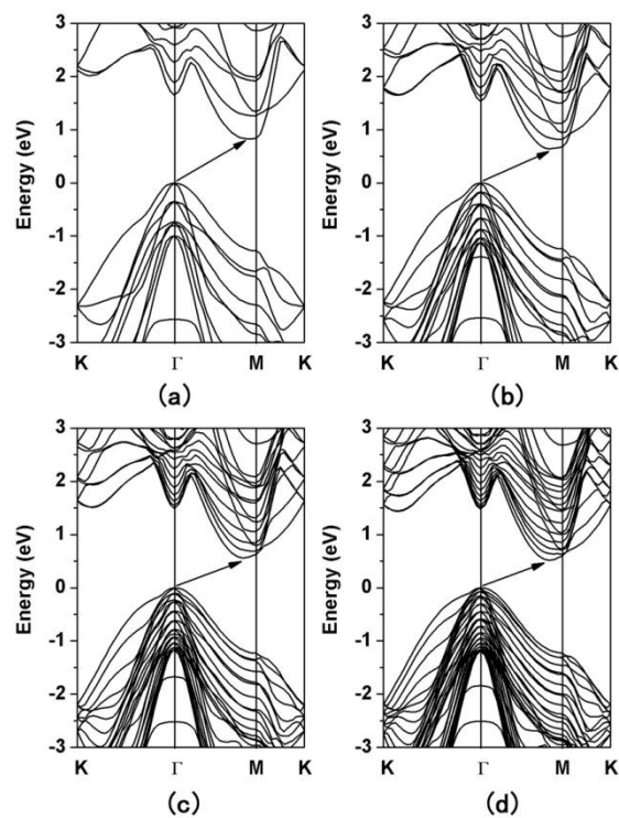
Figure 1s. The band gap structure of Si (111) Layers terminated with only SiH groups on the surface.
