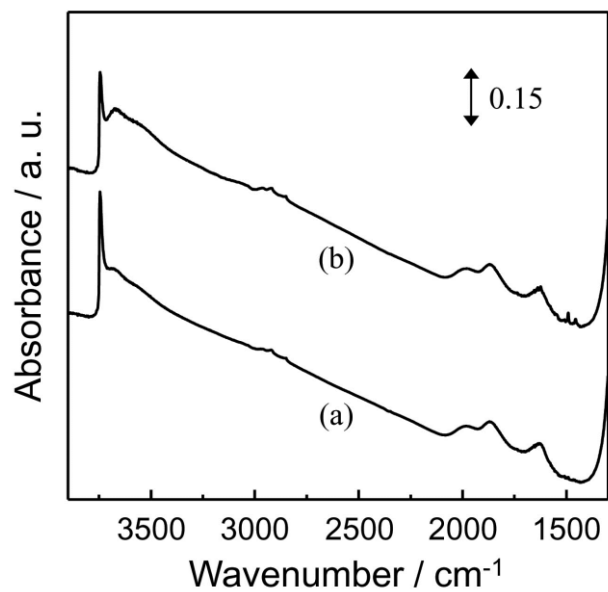
Fig. S3 FT-IR spectra of Al-MMS before pyridine contact (a) and after adsorption of pyridine and subsequent evacuation at 473 K under vacuum (b).
