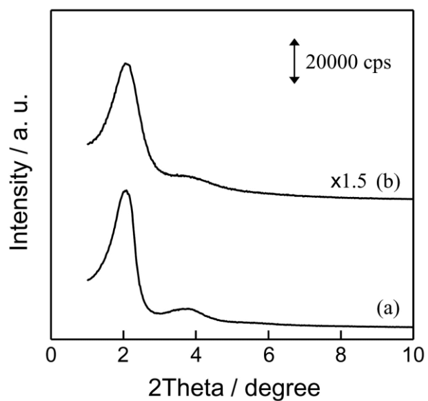
Fig. S2 XRD patterns of (a) Al-MS and (b) Al-MMS.
