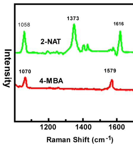
Fig.S5 SERS spectra of 2-NAT and 4-MBA at 10^{-10} M by using Au HS film as a substrate which prepared at 2 wt% of H 2 AuCl 4 on the TSA-doped PANI slice.
