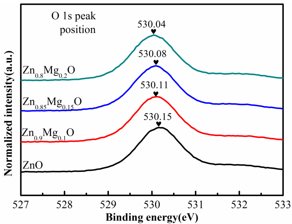
Fig. S1 O 1s peak position evolution for Zn 1-x Mg x O films as a function of Mg composition.
