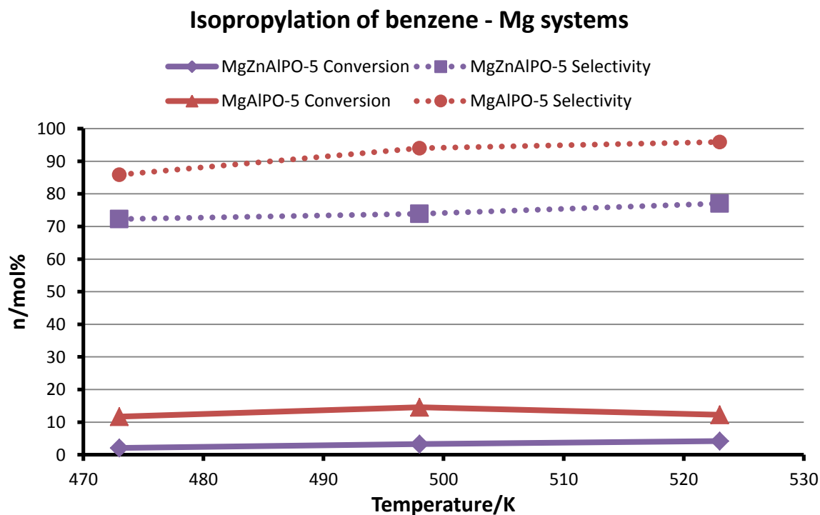
Figure S8: Isopropylation of benzene using Mg-containing AlPO-5 systems. Reaction conditions: WHSV of 3.5 hr -1 , Helium carrier gas of 10 ml/min, feed 6:1 mole ratio of benzene:isopropanol, temperature as shown.
