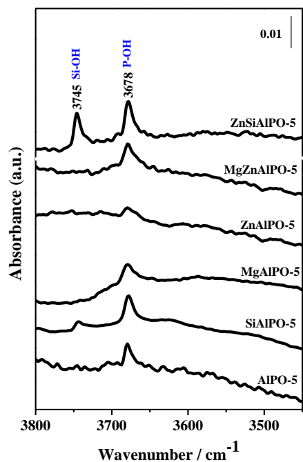
Figure S2: FTIR spectra of the OH stretching region for metal-substituted AlPO-5 systems
