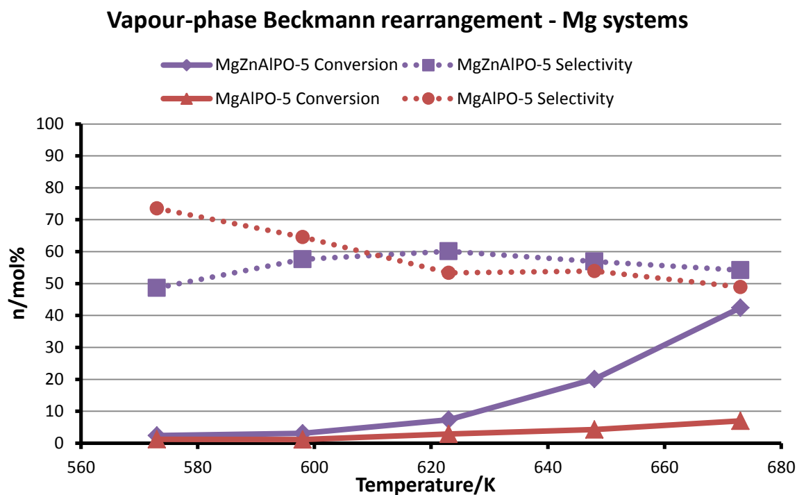
Figure S7: Vapour-phase Beckmann rearrangement of cyclohexanone oxime using Mg-containing AlPO-5 systems. Reaction conditions: WHSV 3.3 hr -1 , Helium carrier gas flow 20 ml/min, 0.3 g of catalyst, liquid feed 300g/l of cyclohexanone oxime in methanol, temperature as shown.
