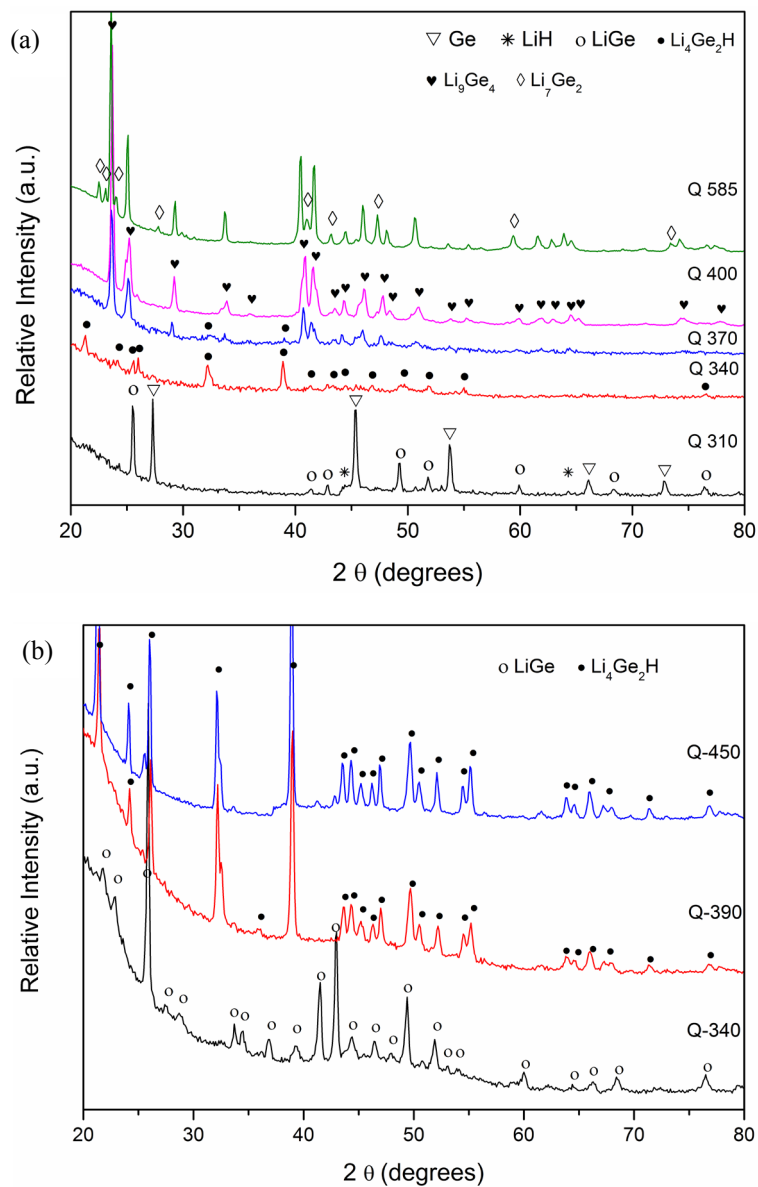
Figure S1. Ex-situ XRD of DSC products of 3LiH/Ge sample heated to (a) 310 °C, 340 °C, 370 °C, 400 °C, and 585 °C under Ar and (b) 340 °C, 390 °C, and 450 °C under H 2 .
