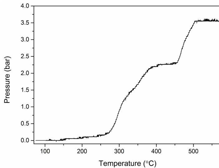
Figure S2. Pressure profile of self-generated deuterium gas of 3LiD/Ge sample during heating up to 600 °C carried under static vacuum PND experiment.
