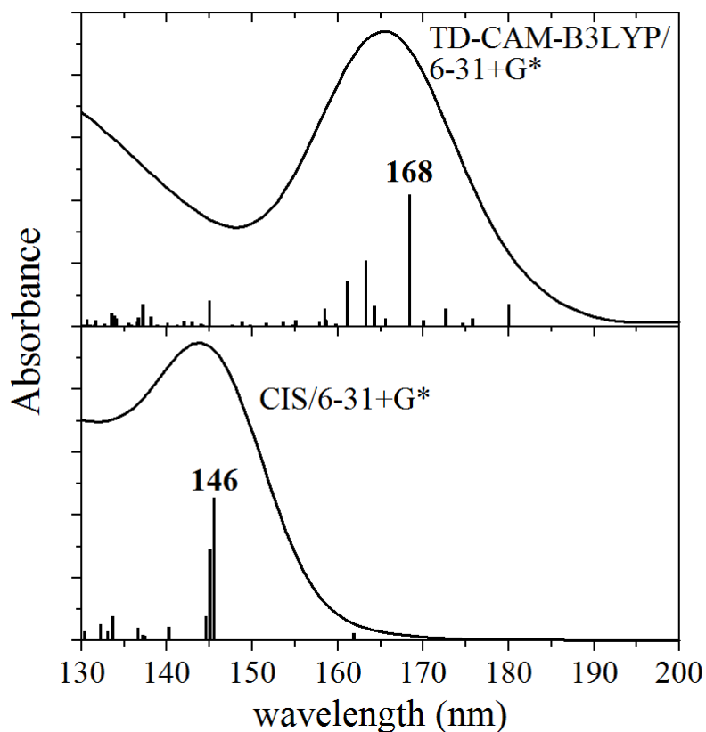
Fig. S1 Calculated electronic absorption spectra of the \text{H}_2\text{N}-(\text{CH}_2-\text{CO}-\text{NH})_3-\text{CH}_2-\text{COOH} \beta -strand.
