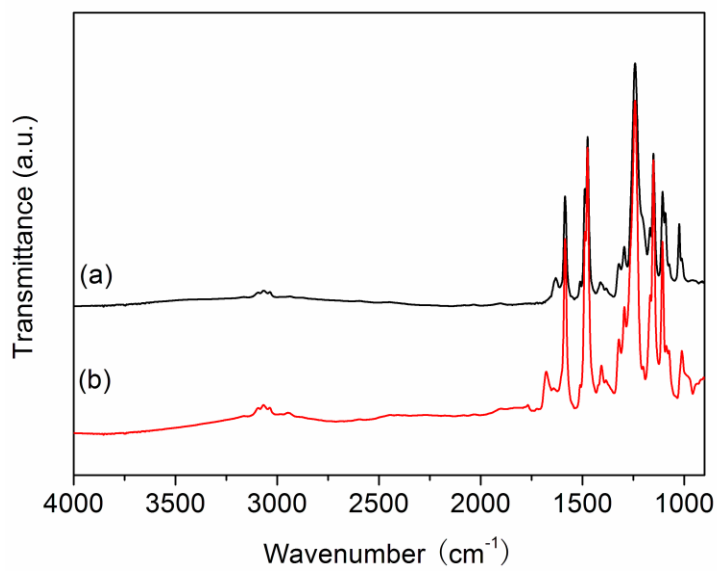
Figure S1. FTIR spectra of (a) S-Radel and (b) degraded S-Radel.
