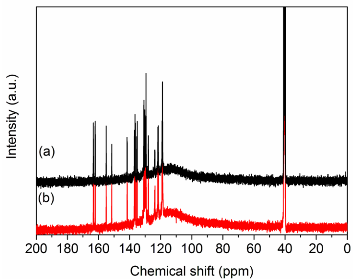
Figure S4. ^{13}\text{C} NMR of (a) S-Radel and (b) degraded S-Radel in \text{DMSO-d}_6 .
