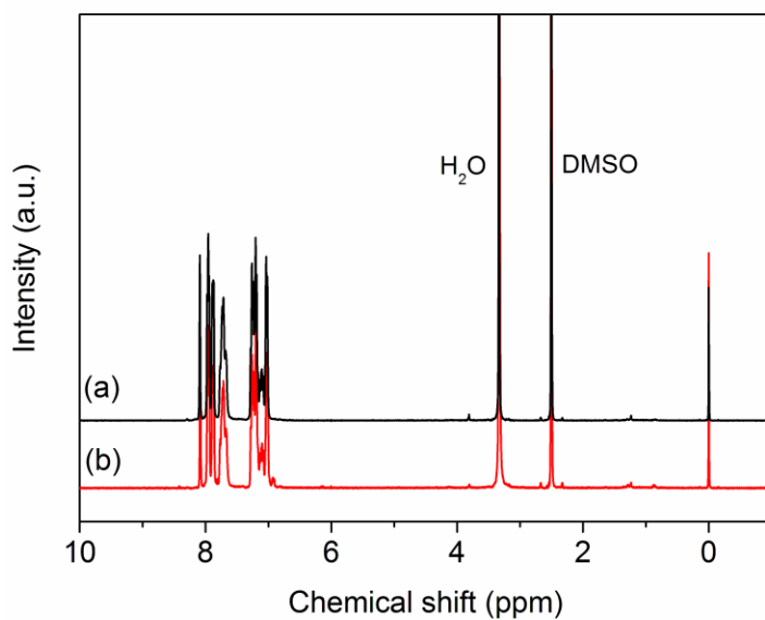
Figure S3. 1 H NMR spectra of (a) S-Radel and (b) degraded S-Radel in DMSO-d 6 .
