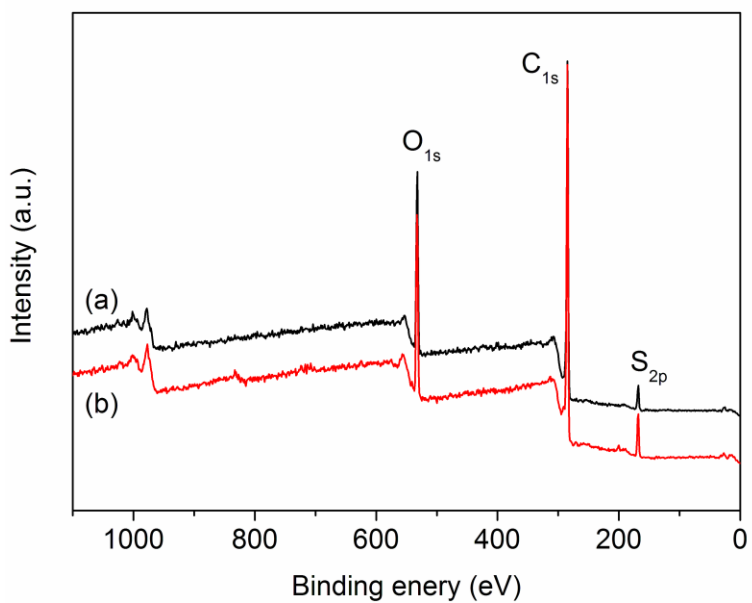
Figure S2. Survey scan XPS spectra of (a) S-Radel and (b) degraded S-Radel.
