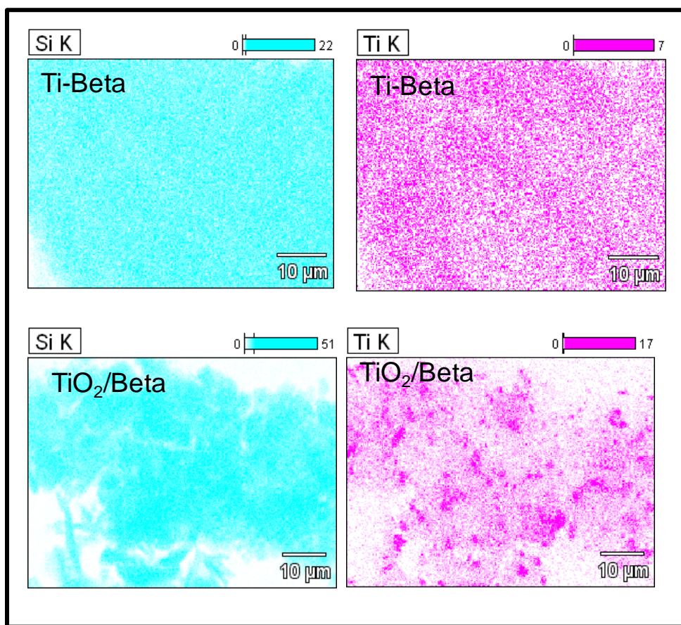
Figure S1. cartographical analysis of Si and Ti in TiO 2 -Beta and SSD TiO 2 /Beta samples.
