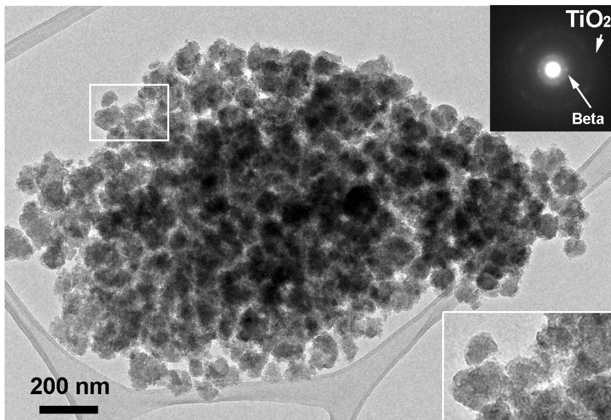
Figure S3. Bright field TEM image showing Beta TiO 2 -Zeolite crystals. The corresponding ED pattern is given as insert at the upper right corner. Enlarged image of the region indicated with rectangle framework is given as insert in the bottom right corner.
