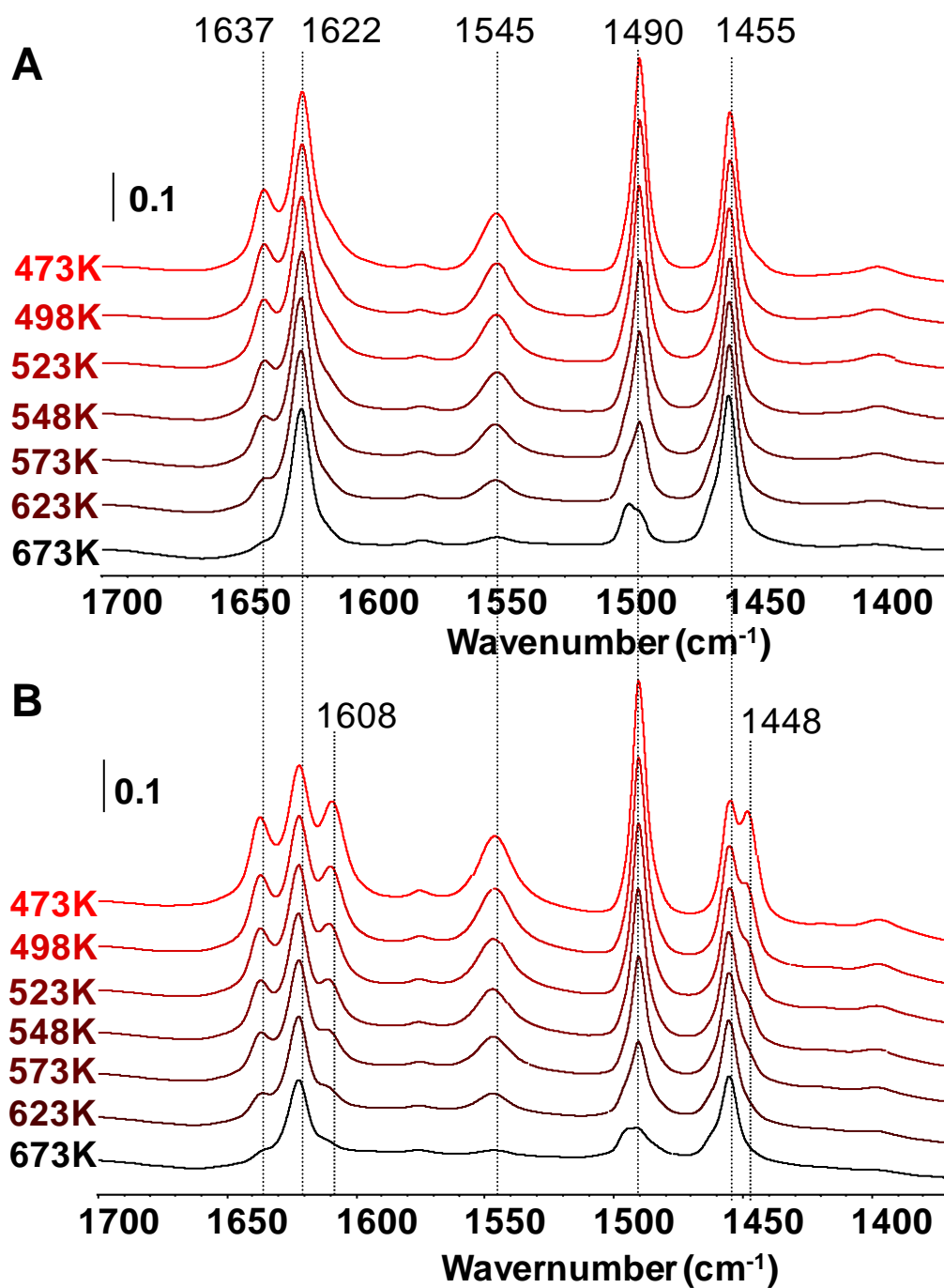
Figure S2. Evolution of the IR spectra of Beta (A) and TiO 2 -Beta (B) during Py desorption under vacuum at different temperature.
