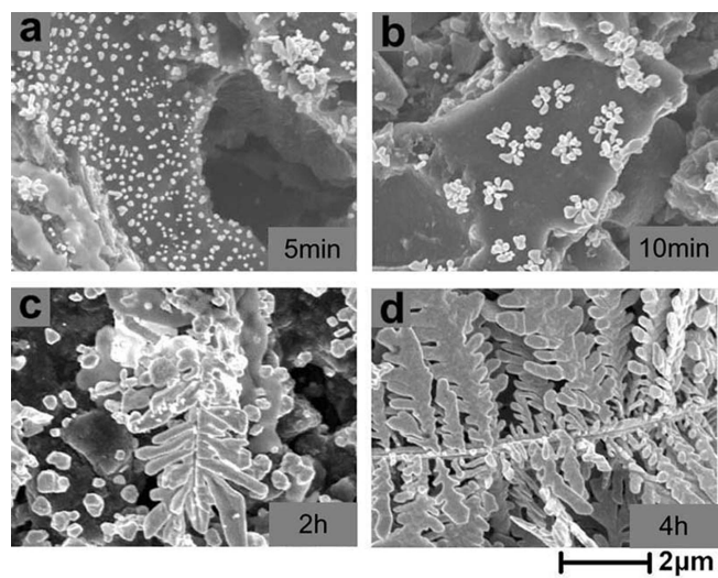
S. Fig. 1 SEM images of MACs surfaces after immersing in 100 ppm AgNO 3 solution for different time without Cl - , PO 4 3- , or SO 4 2- ions absorbed in prior.
