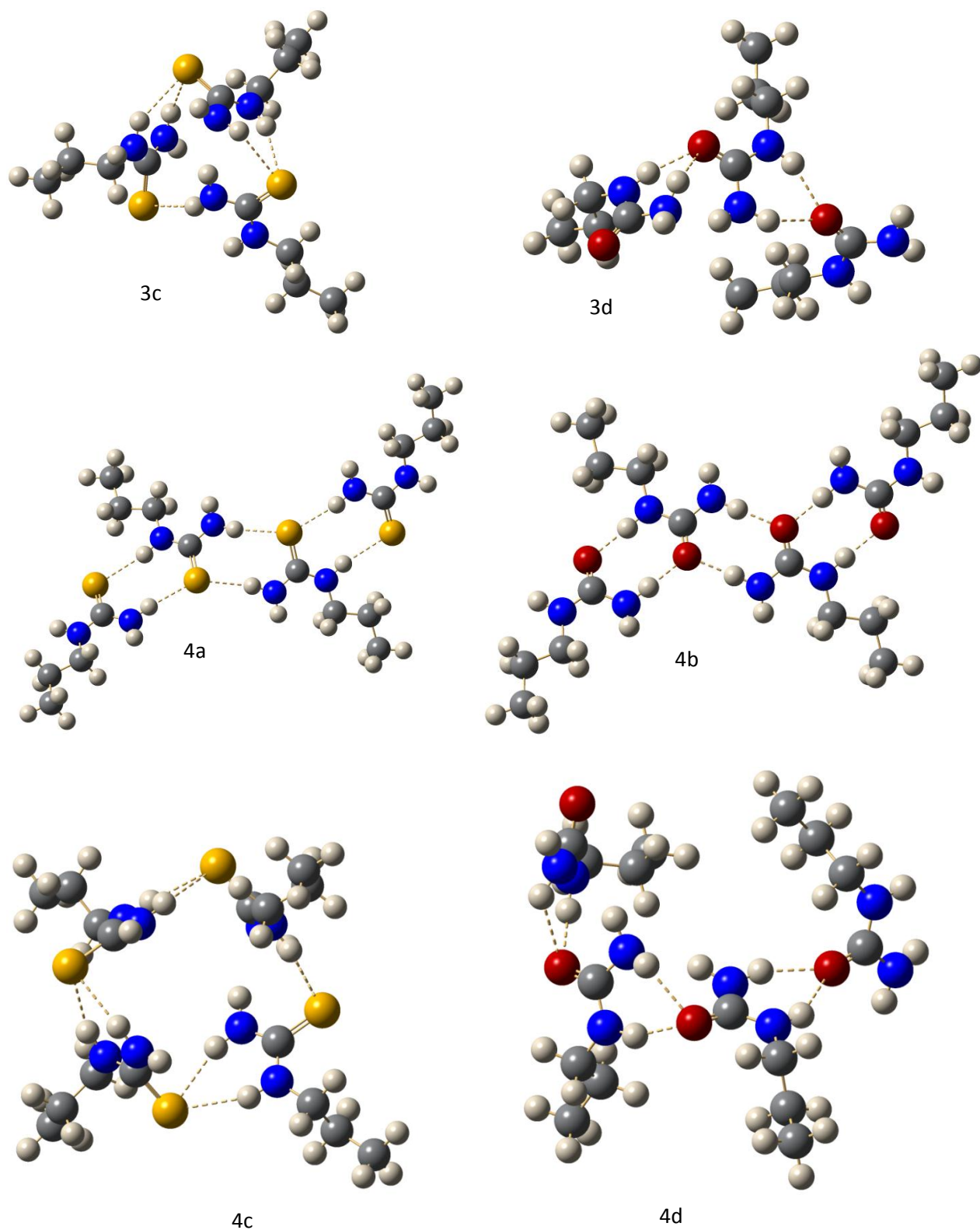
Schema 1S Calculated conformers of N-propylurea (NPU) and N-propylthiourea (NPTU): monomers (1), dimers (2), trimers (3), tetramers (4): cis: a –NPTU, b-NPU; trans: c-NPTU, d-NPU;
