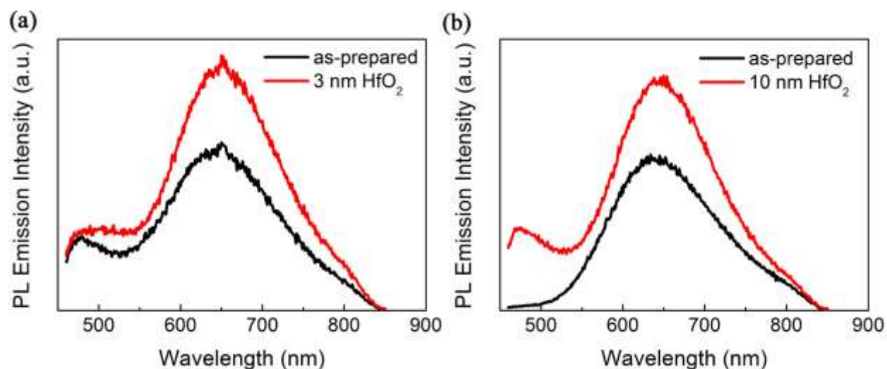
Figure S1. Room temperature PL spectra of the as-prepared and HfO 2 -coated porous Si NWs with different coating thickness: (a) 3 nm, and (b) 10 nm.
