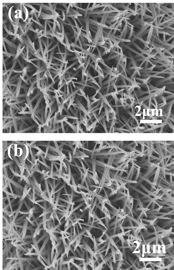
Fig. S1 Typical SEM images of the precursor at different temperature: (a) 105 °C; (b) 115 °C.
