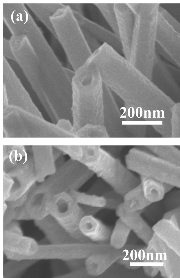
Fig. S2 Typical SEM images of the final samples prepared at different temperature in step 2: (a) 140 °C; (b) 160 °C.
