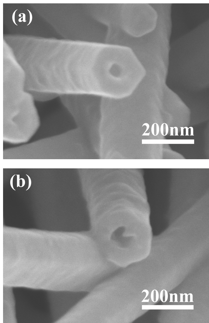
Fig. S3 Typical SEM images of the final samples prepared with different heating time in step 2: (a) 4 h; (b) 8 h.
