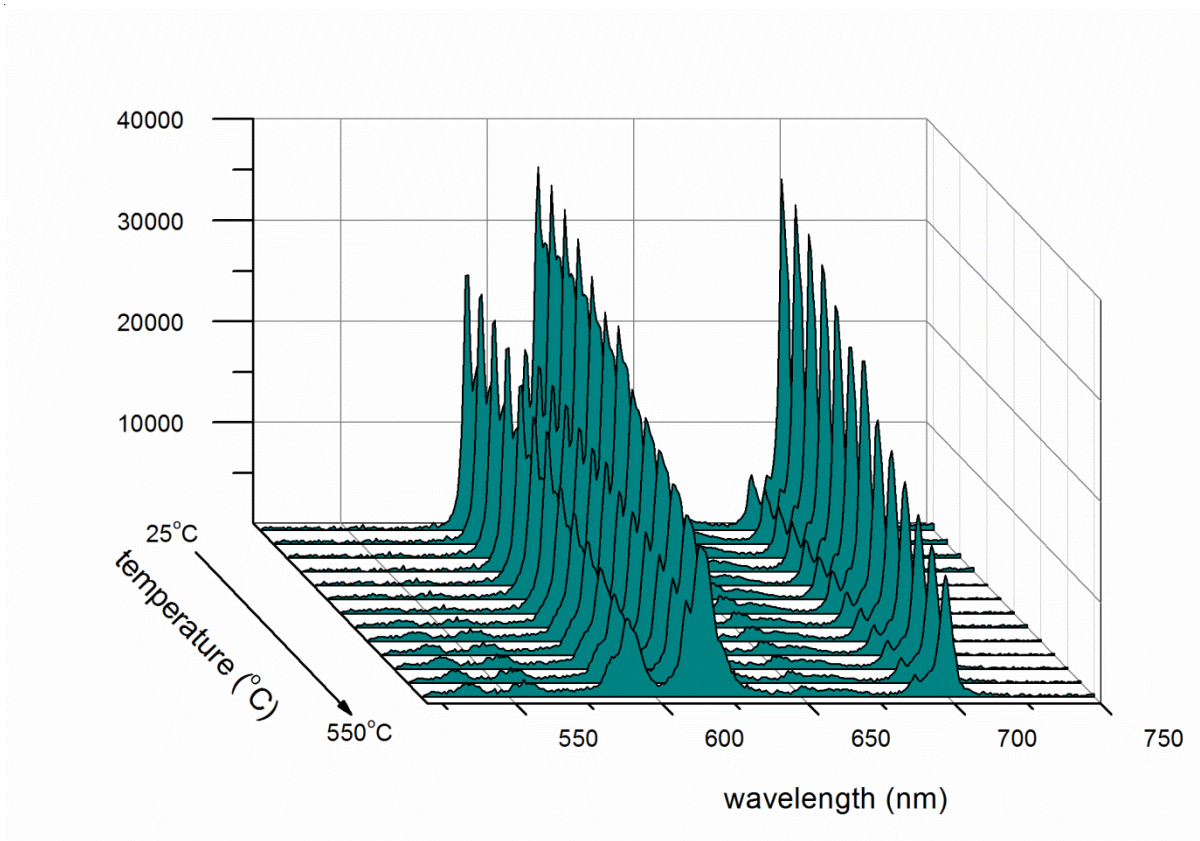
Figure 3_S. The emission spectra of KCa(PO 3 ) 3 doped with Eu 3+ ions in function of surrounding temperature.
