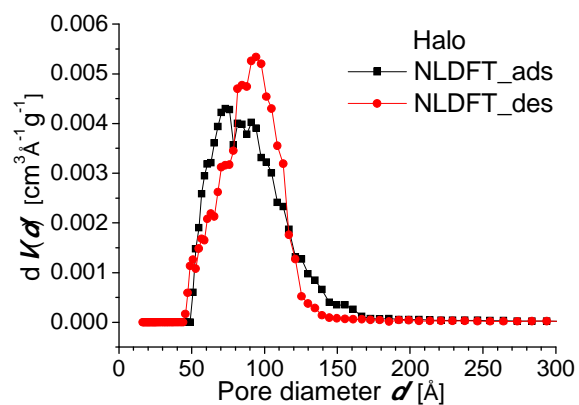
Fig. S1 Pore size distributions of the core-shell Halo particles derived from the adsorption and desorption branch of the nitrogen physisorption isotherm by means of the NLDFT method with a cylindrical pore model for the system nitrogen (77 K)/silica.
