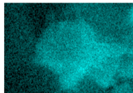
C K
