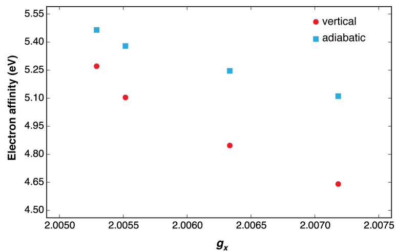
Fig. S4. Correlation between the g_x value of the Y_Z radical and the vertical/adiabatic electron affinity for the models described in Table 1 of the main text.
