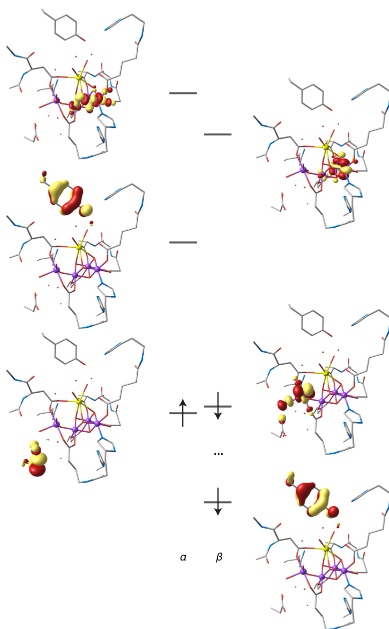
Fig. S2. Frontier orbitals of the S_2^B Y_Z model of the OEC.
