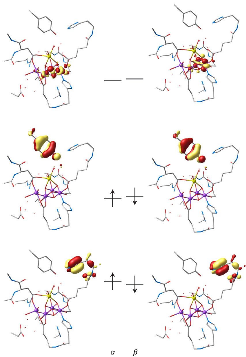
Fig. S1. Frontier orbitals of the S_2^B model of the OEC.
