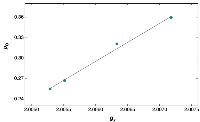
Fig. S3. Correlation between the g_x value of the Y_Z radical and the spin population of the tyrosyl O atom. The models used are those described in Table 1 of the main text.
