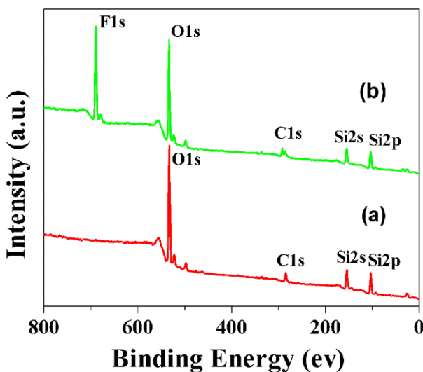
Fig. S1 XPS survey spectra of mesoporous silica coatings before and after fluoroalkyl-grafting (a) F07N and (b) F07NF.
