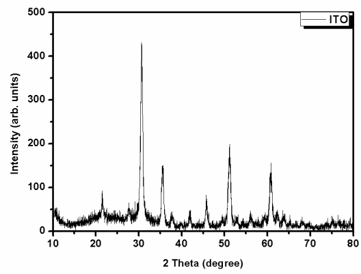
Figure S1 XRD pattern of ITO nanoparticles.
