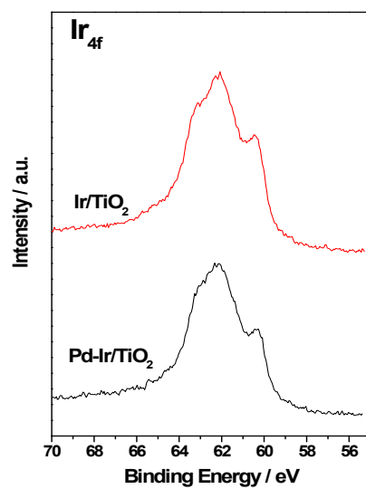
Fig. S2 Ir 4f XPS of Ir/TiO 2 and Pd-Ir/TiO 2 after the reactions.
