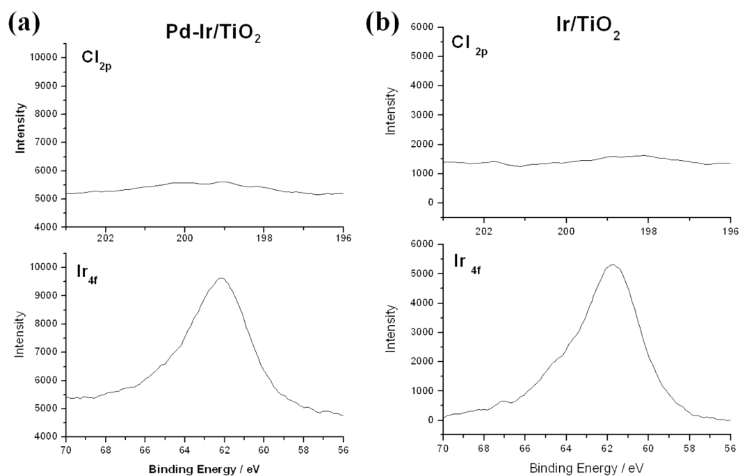
Fig. S1 Cl 2p XPS of (a) Pd-Ir/TiO 2 and (b) Ir/TiO 2 with Ir 4f XPS as comparison.
