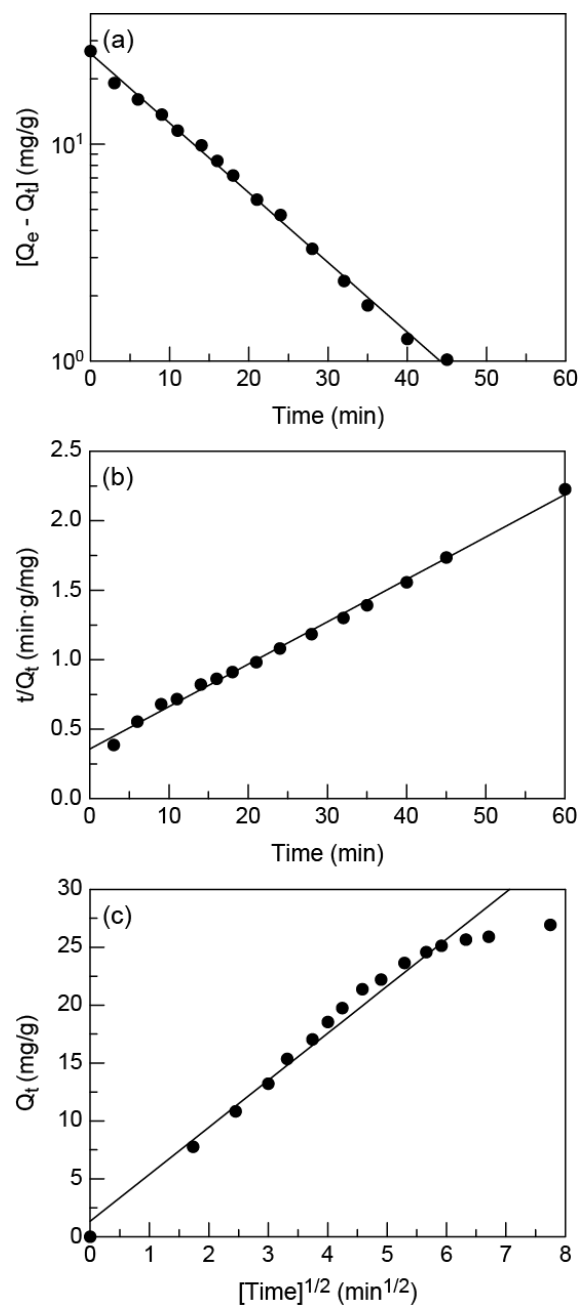
Fig. S2 (a) Pseudo-first, (b) pseudo-second order, and (c) intraparticle diffusion kinetics of adsorption of AG by Cs/PPy/Fe 3 O 4 nanocomposite.
