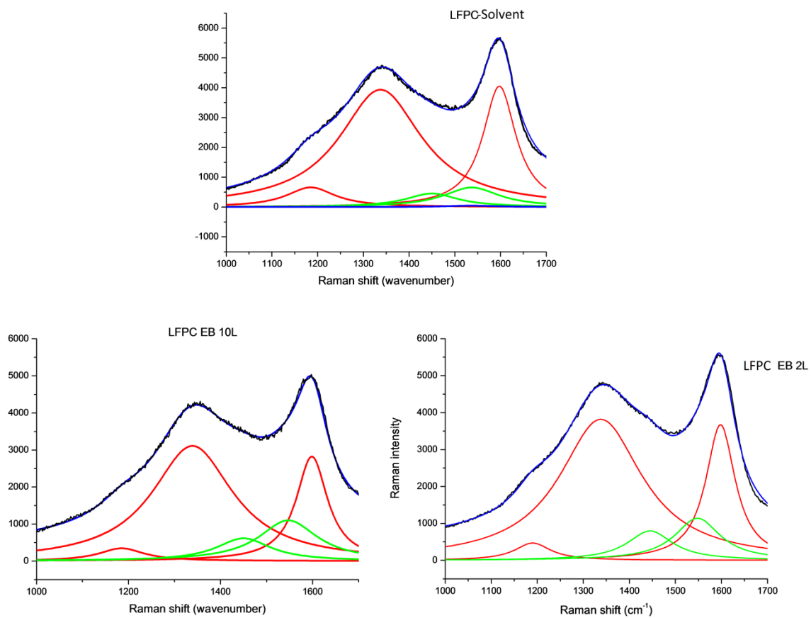
Figure S3. Comparison of the decomposition of the three Raman spectra excited at 633 nm obtained for LFPC-solvent, LFPC-EB-2L and LFPC-EB-10L.
