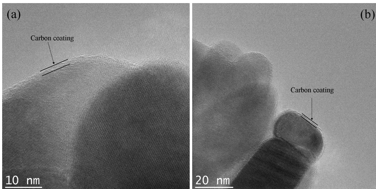
Figure S2. HRTEM images of (a and b) pristine LFPC.
