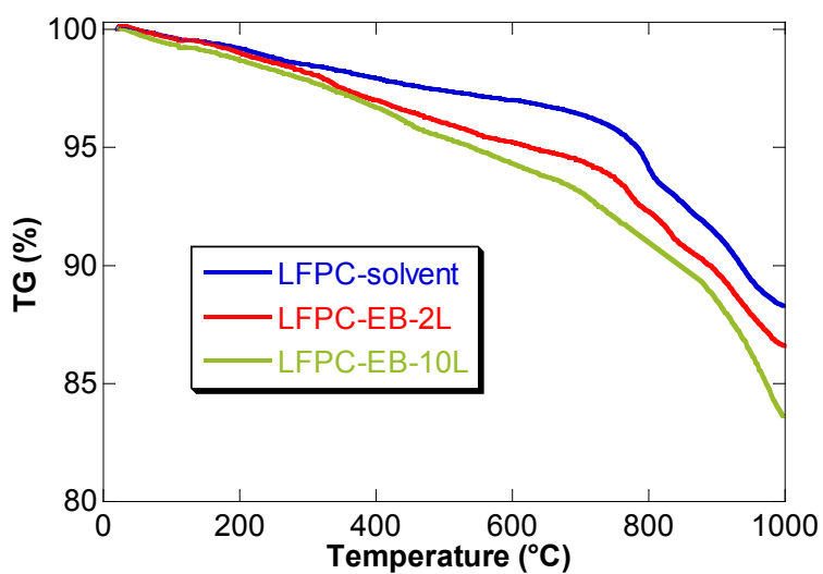
Figure S1. Thermogravimetric curves of LFPC-solvent, LFPC-EB-2L and LFPC-EB-10L.
