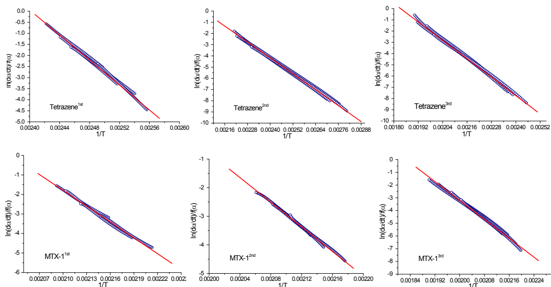
Fig. S1, The combined kinetic analysis plots for non-isothermal decomposition data of MTX-1 and Tetrazene
