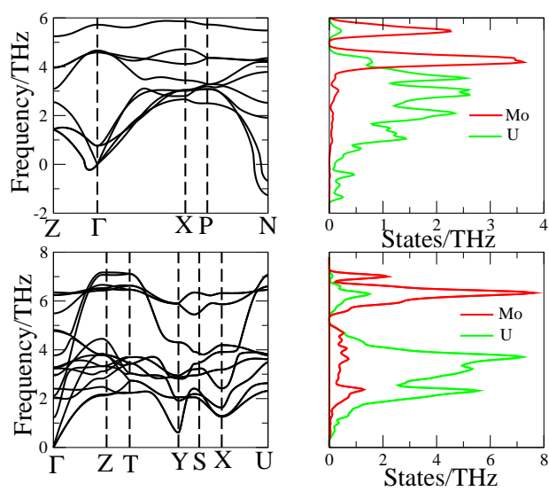
Fig.S1 (color online) The calculated phonon spectra and DOS of the I4/mmm (upper panels) and the Pmmn phases (lower panels) within DFT+D
