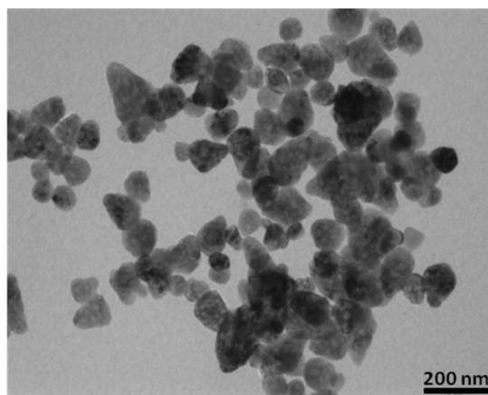
Figure S1. TEM image of ZnO calcined at 550°C
