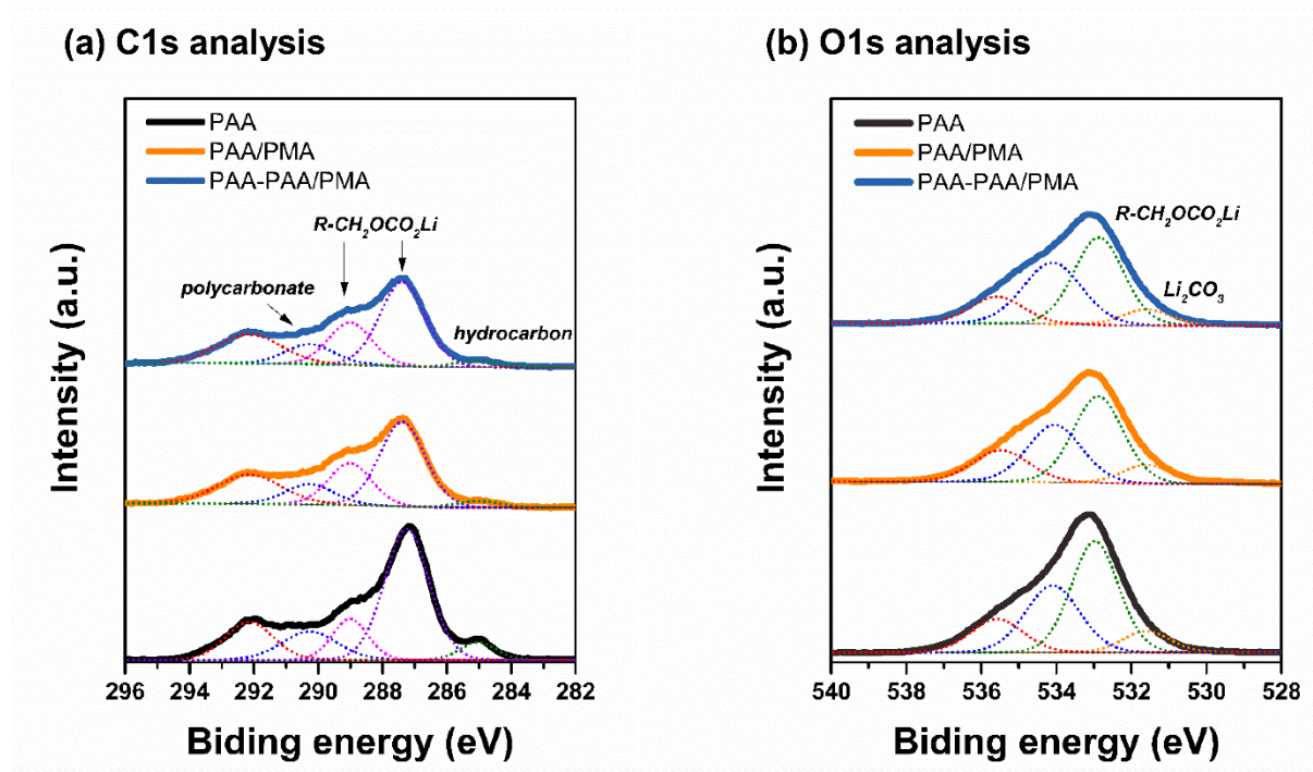
Fig. S1 XPS analytical results for cycled electrode with (a) C1s, and (b) O1s
