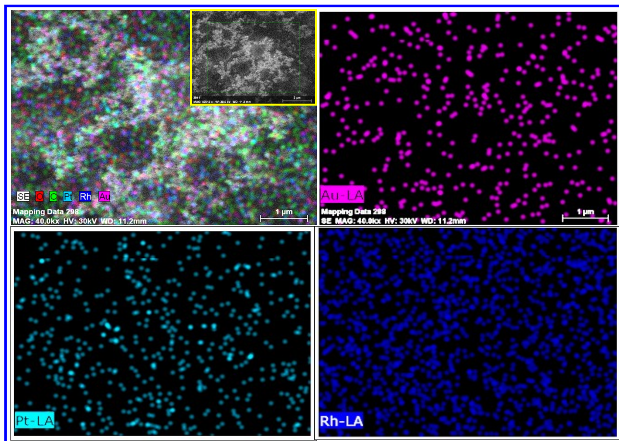
ESI. Field-emission scanning electron microscopic (FE-SEM)/EDX elemental color map overlapping Au, Pt and Rh and EDX elemental color maps of Au, Pt, Rh.
