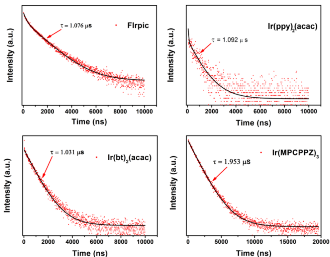
Fig. S1. Transient photoluminescent spectra of the blue, green, orange, and red phosphors singly doped in PVK film excited at 344 nm.
