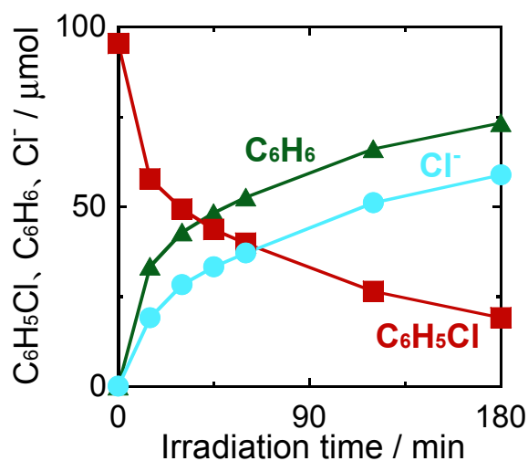
Fig. S1 Time courses of the amounts of chlorobenzene (squares), benzene (triangles), chloride ion (closed circles) in a 2-propanol suspension of 1.0 wt% Pd-TiO 2 in the absence of NaOH under UV light irradiation.
