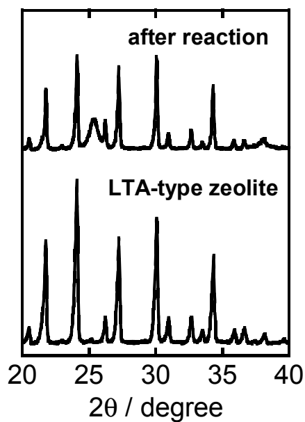
Fig. S2 XRD patterns of fresh LTA-type zeolite and the recovered mixture of LTA-type zeolite and Pd-TiO 2 after the photocatalytic reaction.
